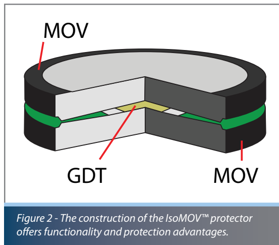
Bourns® IsoMOV™ Hybrid Protector
