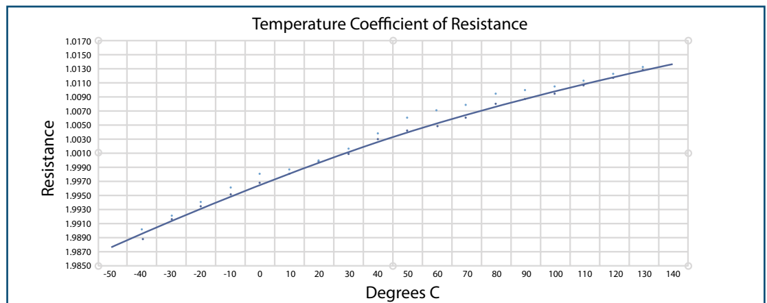
Figure 6. Data from Look Up Table Showing Resistance Drift with Temperature
