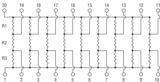
820 ELECTRICAL SCHEMATIC
