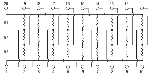
830 ELECTRICAL SCHEMATIC
