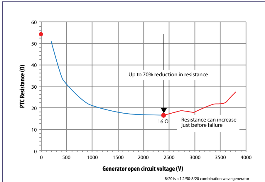
Figure 5. | CMF-RL55-0-A1 Resistance During 8/20 μs Generator Resistance = 2 Ω
