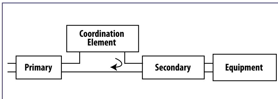
Figure 2. | Current-Type Coordination
