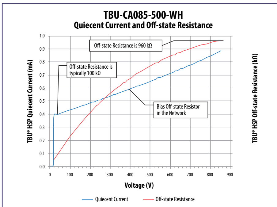
Figure 6. TBU® HSP tripped resistance is ~ 100 kΩ. No blind spots in the current-type coordination
