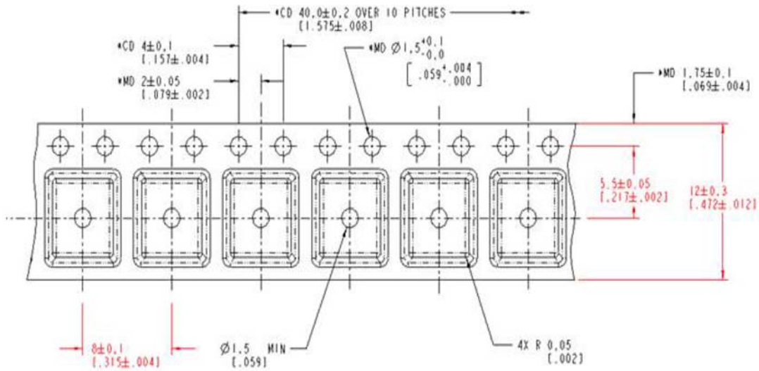
Figure 1: 70ABJ-4-Male Current Design
