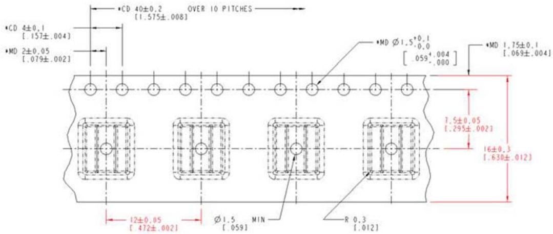
Figure 2: 70ABJ-4-Male Improved Design
