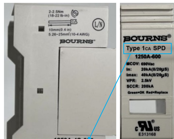
Type 1CA SPD
