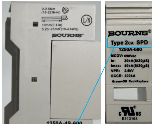
Type 2CA SPD
