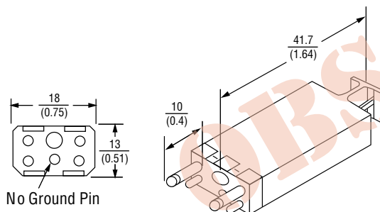
Figure 3 3A-Type Continuity Module
