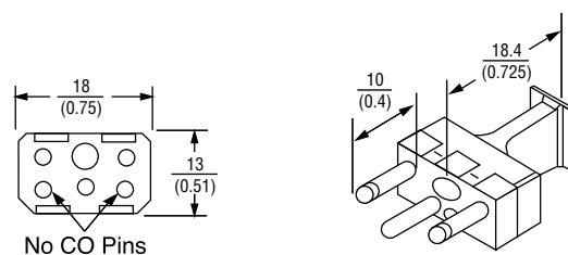
Figure 6 5A-Size Grounding Module
