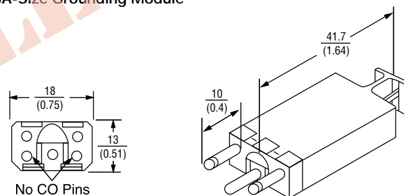
Figure 4 3A-Size Grounding Module
