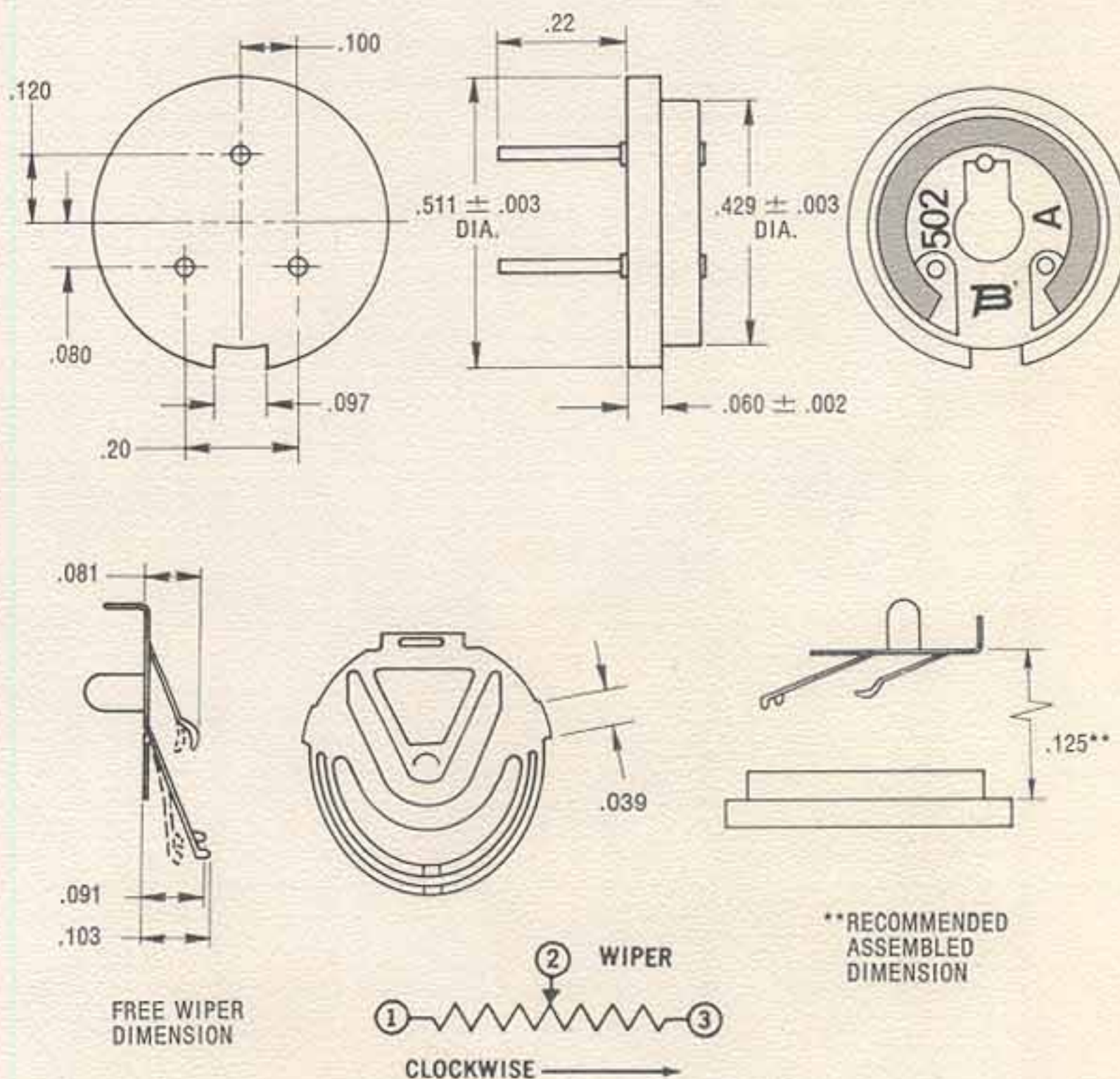
ELEMENT & PIN ASSY.
