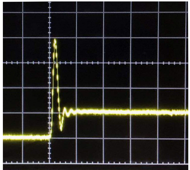
Step response from Fluke 5220A amplifier at 20A square-wave current (no load), 20 \mu\text{s}/\text{div} range
