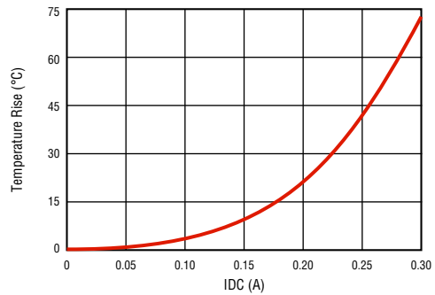
Temperature Rise Plot
