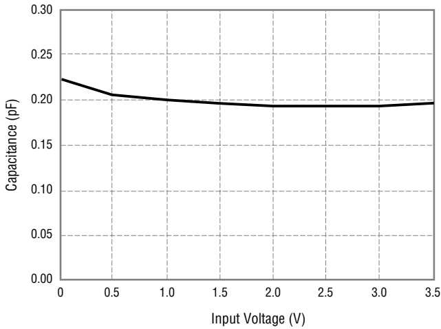
Typical Capacitance Variation of C_{IN} vs V_{IN}
