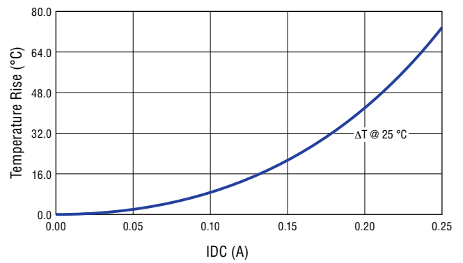
CC322522A-101K
