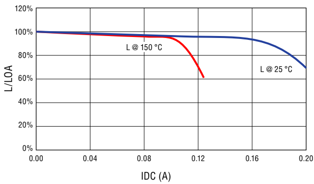
CC322522A-101K
