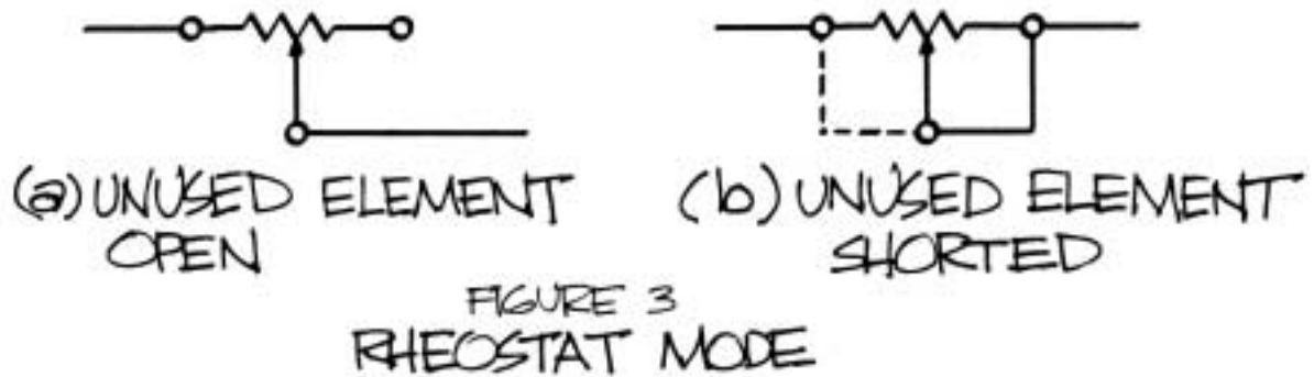
FIGURE 3 RHEOSTAT MODE
