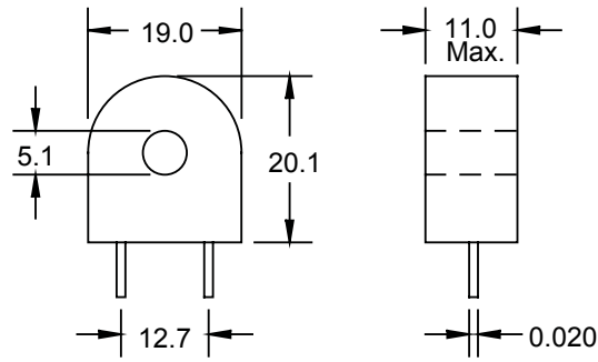
Dimensions: mm
